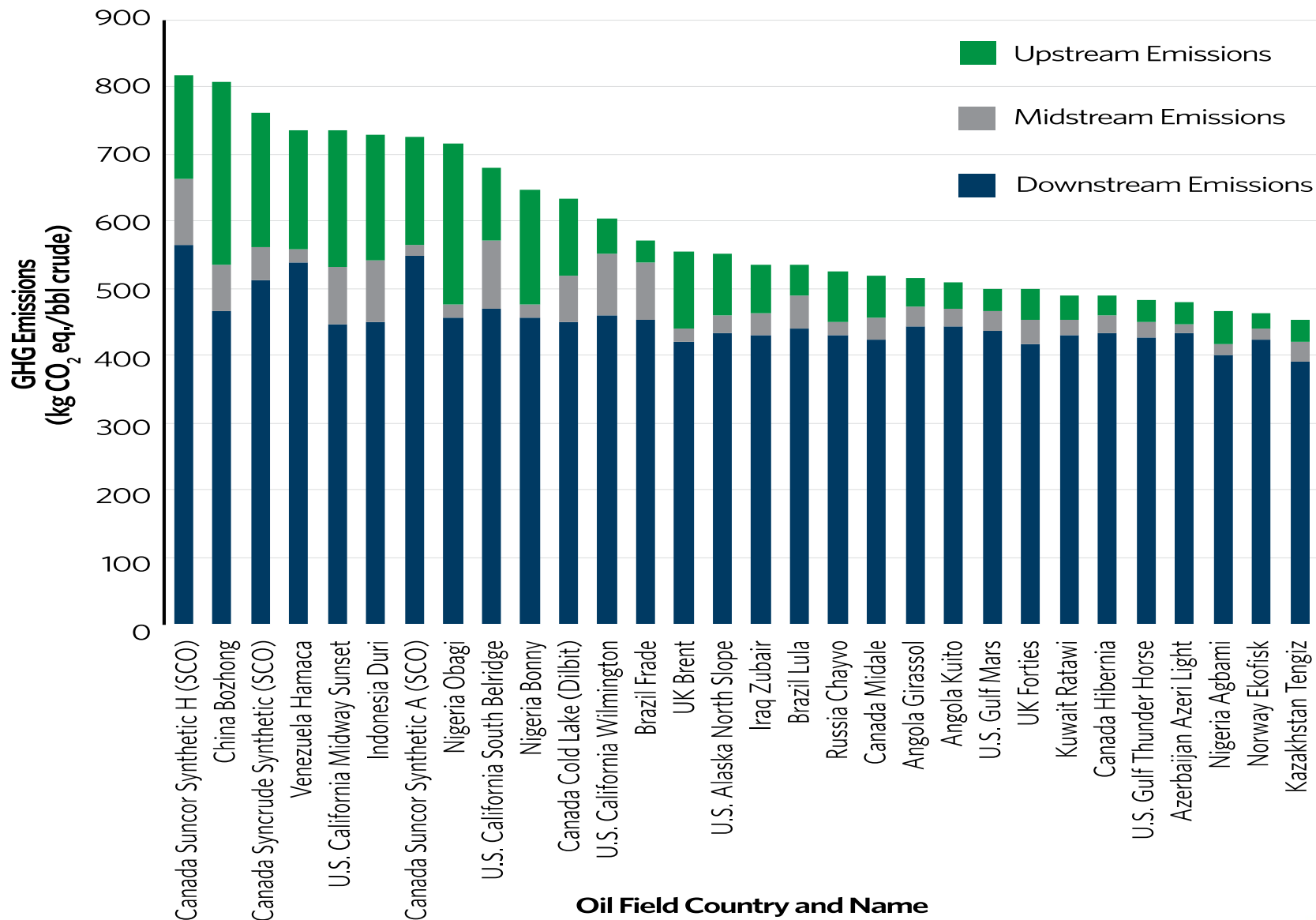
FIGURE 12 Total GHG Emissions for 30 Phase 1 OCI Test Oils
