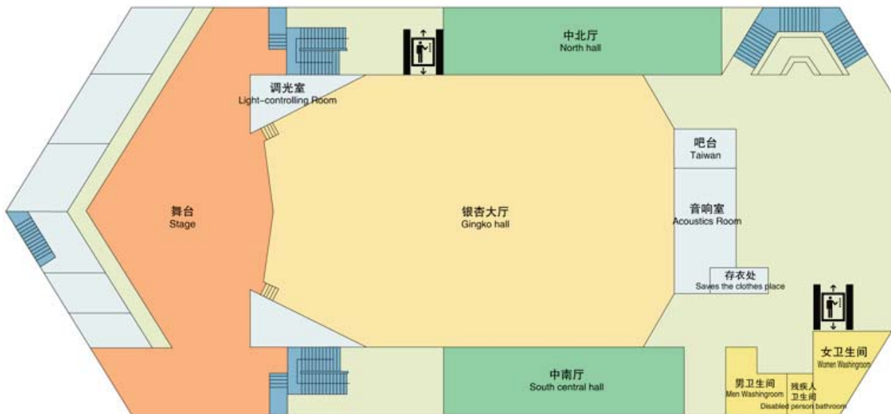
1号楼三层平面示意图 Third Floor Plan of Building No.1
